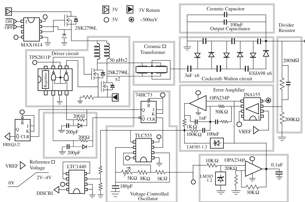
Fig1 Schematic circuit of high voltage power supply
