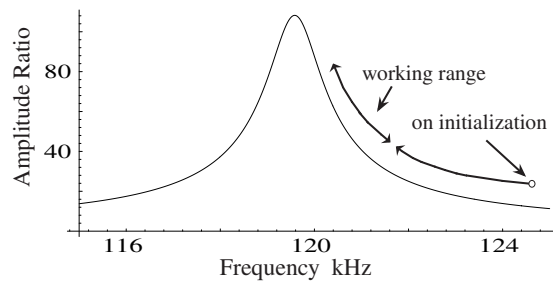
Fig2 Resonance shown by transformer
