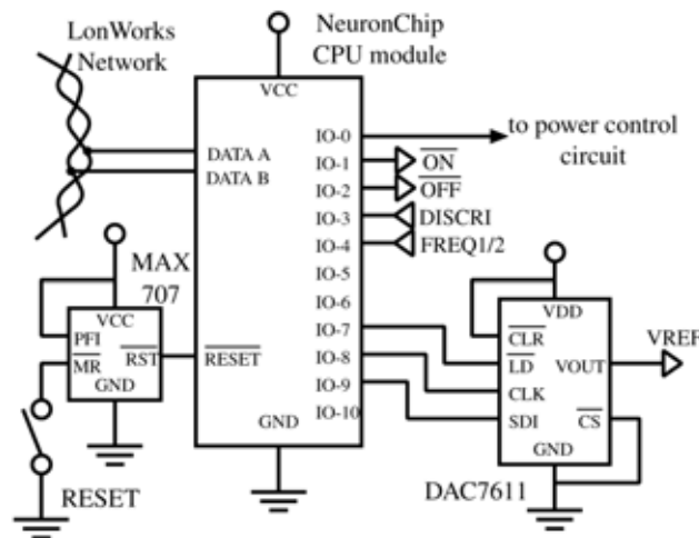
Fig3 Interface circuit between neuron chip and high voltage power supply
