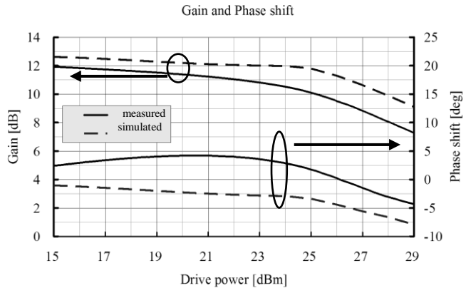
Fig.6 Comparison of simulation and measurement (Gain and Phase shift)
