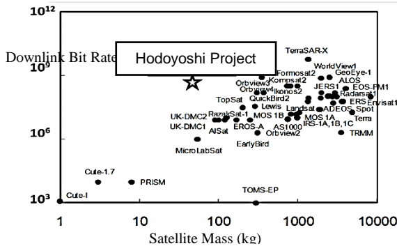
Fig.1 Down link bit rate vs. satellite mass for low earth orbit. ★ denotes presented novel technology.
