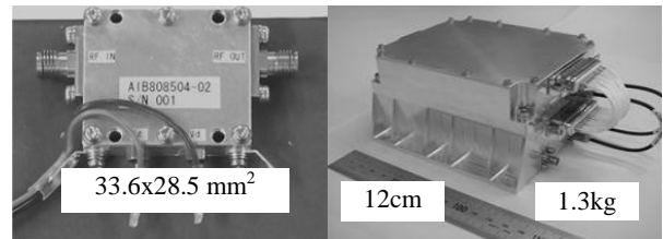
Fig.4 Photograph of PA (left) and transmitter (right)
