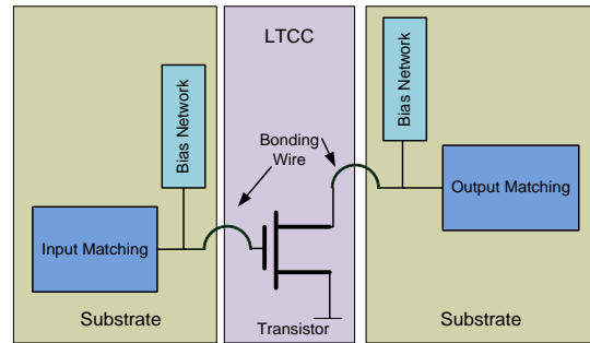
Fig.3 Structure of the Circuit Layout
