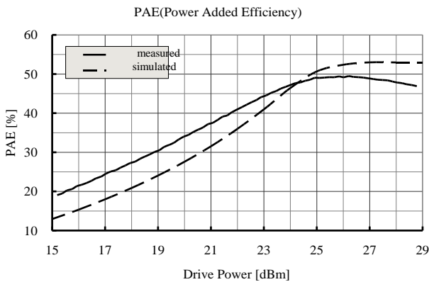
Fig.7 Comparison of simulation and measurement (PAE)
