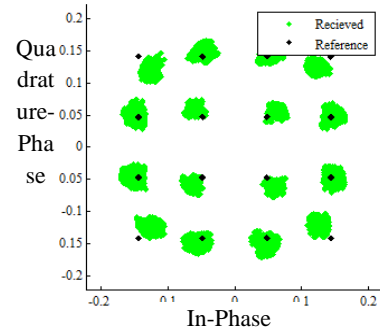
Fig.9 Constellation diagram 100Mbps, W/O noise, 199992 symbols, W/O pre-distortion
