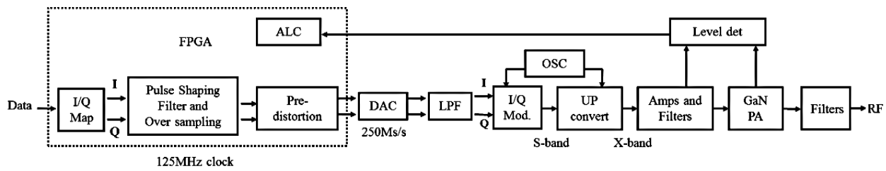
Fig.8 Block diagram of transmitter system (Engineering Model)
