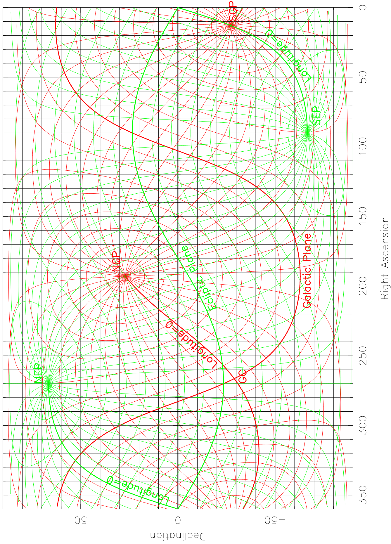
Equatorial—Ecliptic—Galactic Conversion
