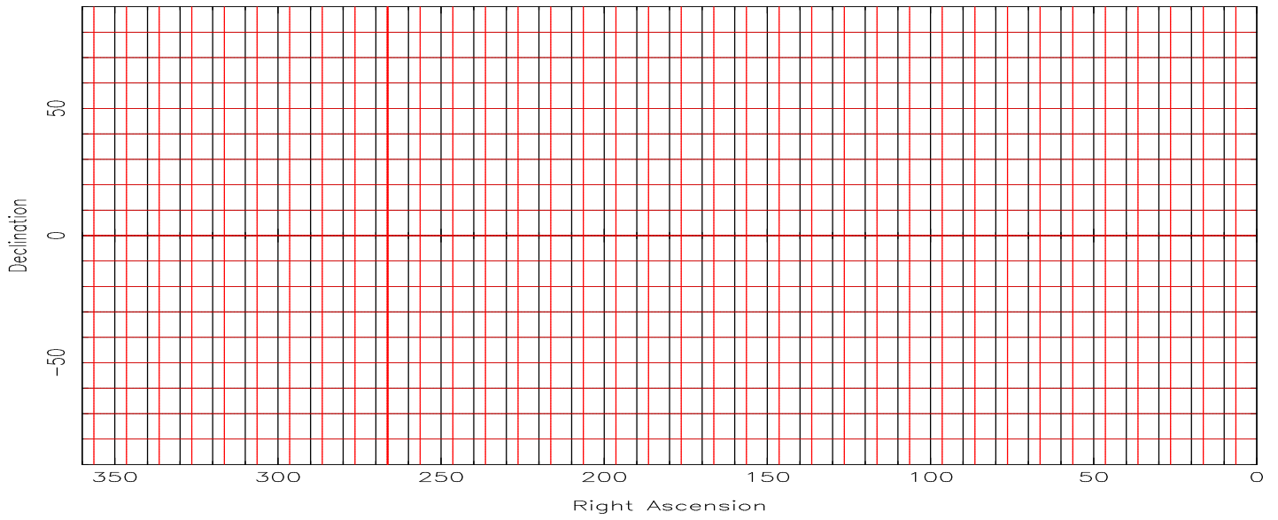
Equatorial-->Galactic Conversion First Step
