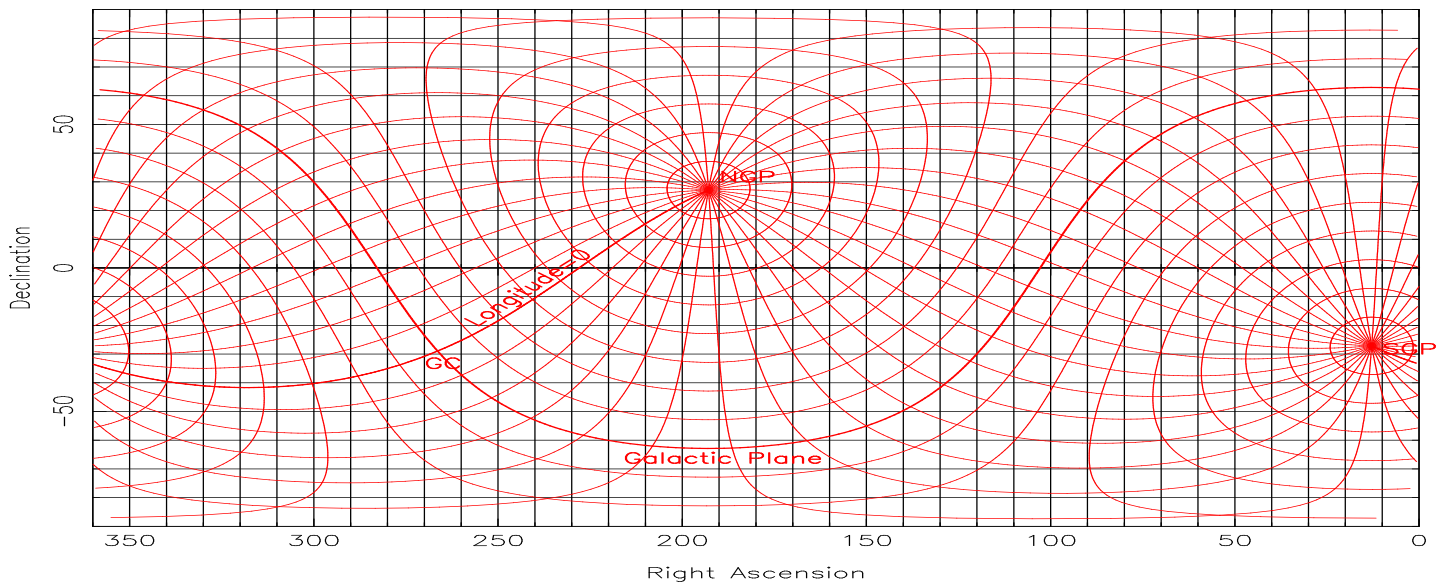
Equatorial-->Galactic Conversion Third Step
