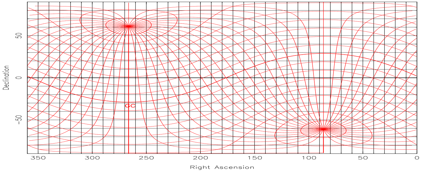
Equatorial-->Galactic Conversion Second Step
