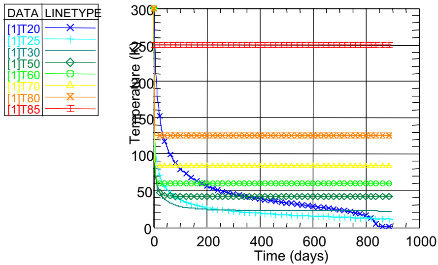
Fig. 5: Initial cooldown time for the HII/L2 cryogenic system without a 20 K cooler
