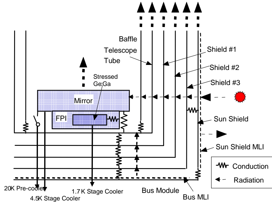
Fig. 1: Schematic drawing of the cryogenic system
