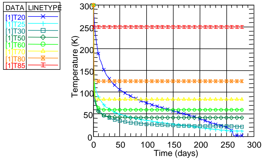
Fig. 4: Initial cooldown time for the HII/L2 cryogenic system with a 20 K cooler
