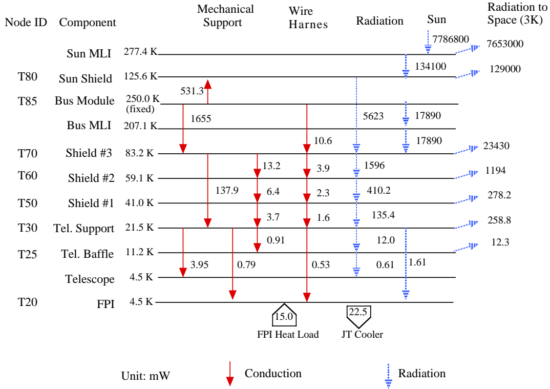
Fig. 3: Heat flow in the HII/L2 cryogenic system
