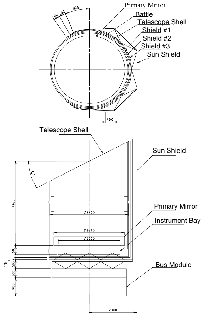
Fig. 2: Cutaway view of the cryogenic system
