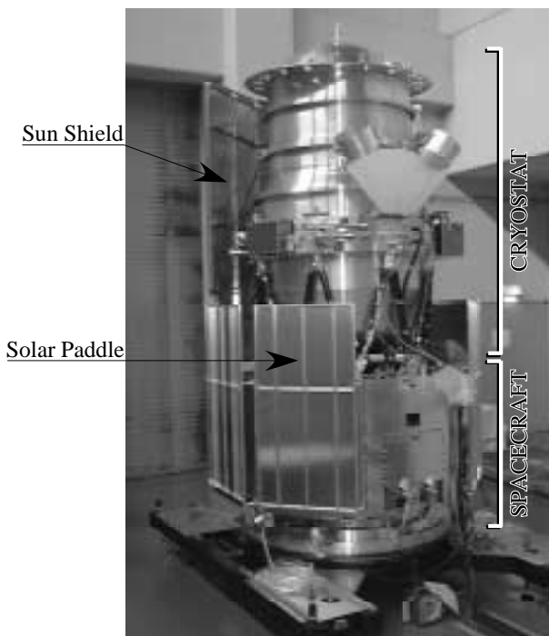
Fig. 1: Mechanical Test Model (MTM) of the ASTRO-F. This model simulates the launch configuration of the ASTRO-F. The cryostat which contains the telescope system and the focal-plane instruments is put on the spacecraft. The total height is approximately 3.7 m. The solar paddle and the sun shield are also seen (just mass dummies).
