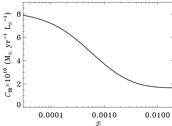
Fig. 1: C_{\text{IR}} (conversion coefficient from the dust luminosity to the star formation rate) as a function of the dust-to-gas ratio, \mathcal{D} .
