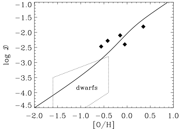
Fig. 2: Relation between the dust-to-gas ratio \mathcal{D} and oxygen abundance [O/H] . The solid line represents the well-fitted model by Hirashita (1999a, b). The observed relations for nearby spiral galaxies are presented with the square Issa et al. (1990). The area marked with dwarfs represents a typical locus of dwarf irregular galaxies and blue compact dwarf galaxies (Lisenfeld & Ferrara 1998).
