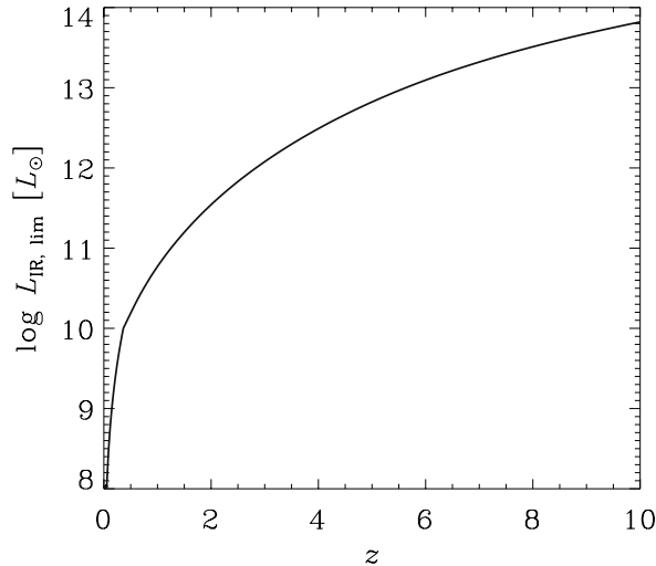
Fig. 4: Minimum of the detected IR luminosity as a function of z . The detection limit of HII/L2 is applied.
