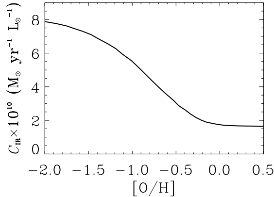
Fig. 3: C_{\text{IR}} (conversion coefficient from the dust luminosity to the star formation rate) as a function of the oxygen abundance, [\text{O}/\text{H}] .
