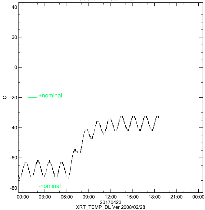
Radiator: HKU_RAD_TMP
